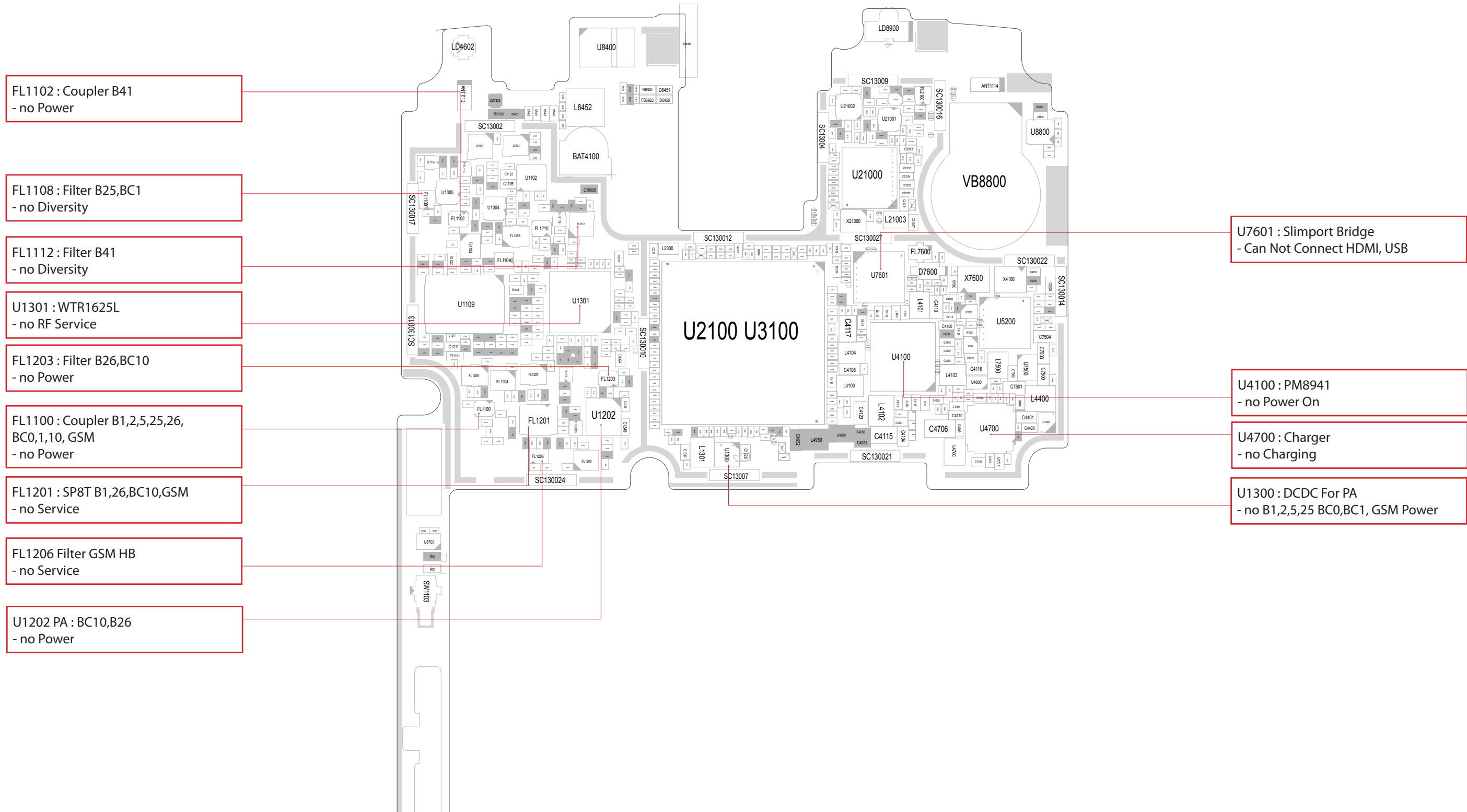
LG-LS990-MAIN_EAX65632401_1.0_TOP-2
